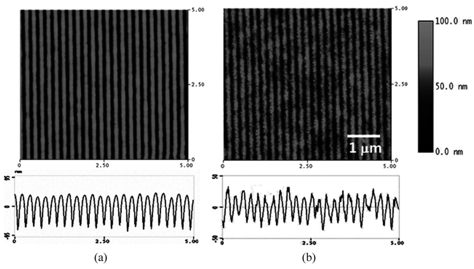
Figure 1. AFM image of (a) the NOA 81 film after NIL and (b) the NOA 81 film coated ITO.
